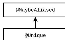
Figure 27.1: Type hierarchy for the Aliasing type system. These qualifiers are applicable to any reference (non-primitive) type.
