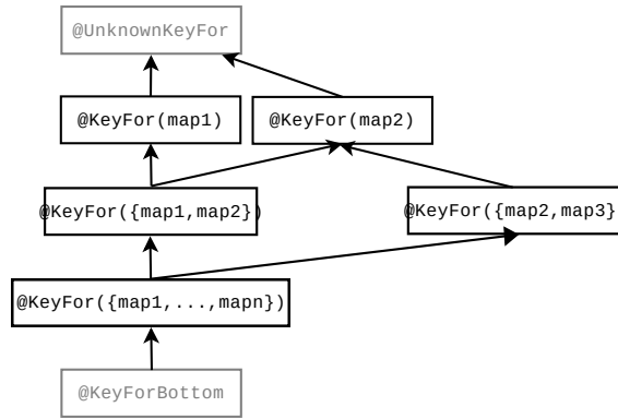
Figure 4.1: The subtyping relationship of the Map Key Checker’s qualifiers. @KeyFor (A) is a supertype of @KeyFor (B) if and only if A is a subset of B . Qualifiers in gray are used internally by the type system but should never be written by a programmer.
