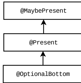
Figure 5.1: The subtyping relationship of the Optional Checker’s qualifiers.
