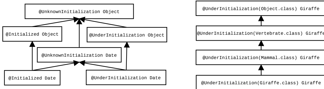
Figure 3.4: Partial type hierarchy for the Initialization type system. @UnknownInitialization and @UnderInitialization each take an optional parameter indicating how far initialization has proceeded, and the right side of the figure illustrates its type hierarchy in more detail.
